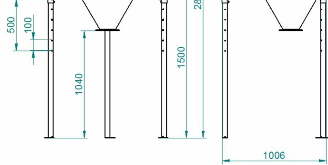
Dimensions with 1 500 mm legs
